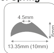
10mm Glass PG-201
