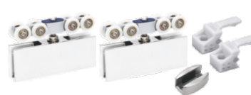
LSL-44-R8 (Set) 8 Wheel Rectangular 2 Set Roller (Brass), 2 Stopper 1 Floor Guide
